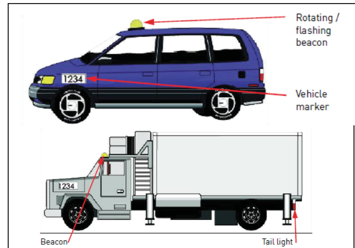
Beacons and vehicle markers shall be placed as shown.
